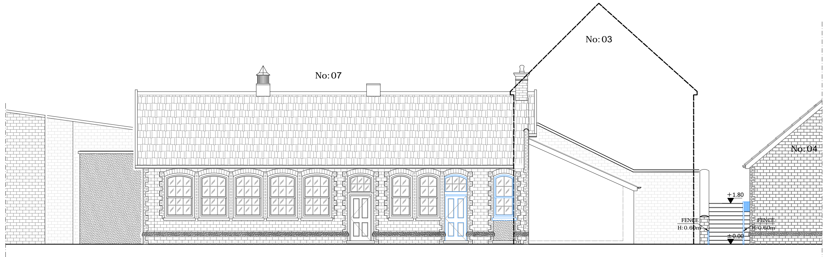
PROPOSED FRONT ELEVATION SCALE: 1/100
